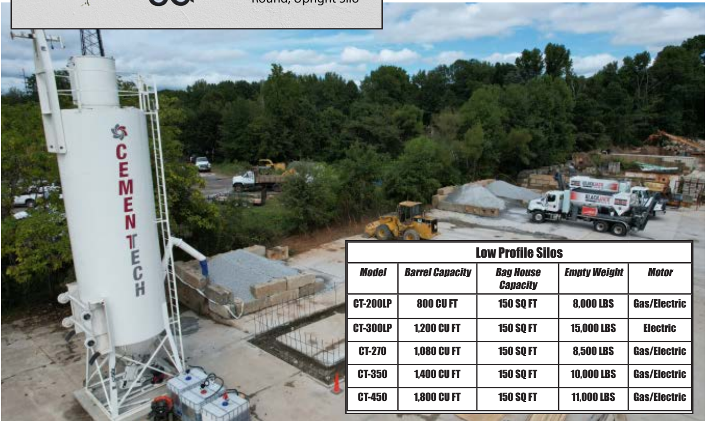
Round, Upright Silo
